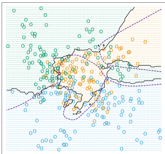
15-Nearest Neighbors
