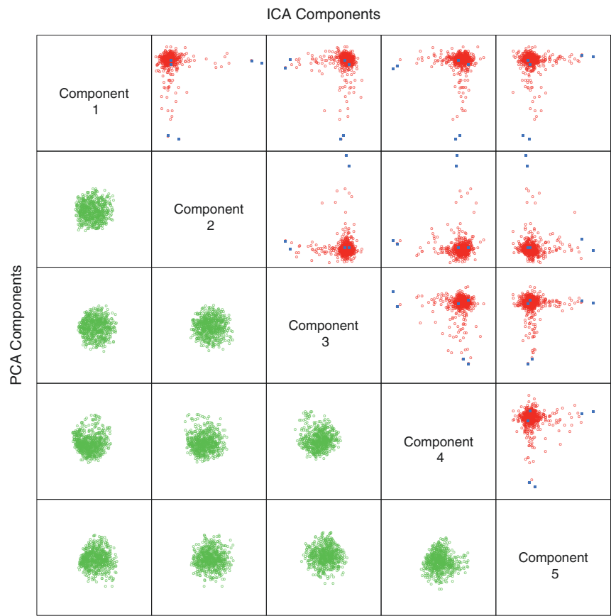
FIGURE 14.39. A comparison of the first five ICA components computed using FastICA (above diagonal) with the first five PCA components(below diagonal). Each component is standardized to have unit variance.
