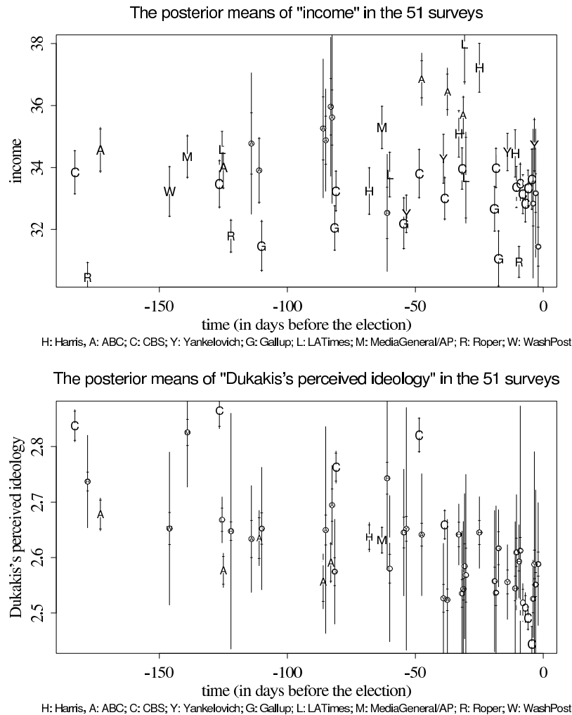
Figure 18.2 Estimates and standard error bars for the population mean response for two questions: (a) income (in thousands of dollars), and (b) perceived ideology of Dukakis (on a 1–7 scale from liberal to conservative), over time. Each symbol represents a different survey, with different letters indicating different survey organizations. The size of the letter indicates the number of responses to the question, with large-sized letters for surveys with nearly complete response and small-sized letters for surveys with few responses. Circled letters indicate surveys for which the question was not asked; the estimates for these surveys have much larger standard errors. The inner brackets on the vertical bars show the within-imputation standard deviation for the average from each poll.
