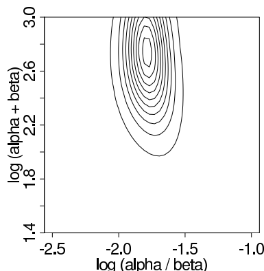
Figure 5.2 First try at a contour plot of the marginal posterior density of (\log(\frac{\alpha}{\beta}), \log(\alpha+\beta)) for the rat tumor example. Contour lines are at 0.05, 0.15, ..., 0.95 times the density at the mode.
