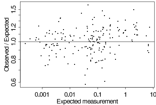
Figure 19.9 Observed PERC concentrations (for all individuals in the study) divided by expected concentrations, plotted vs. expected concentrations. The x and y-axes are on different (logarithmic) scales: observations vary by a factor of 10,000, but the relative errors are mostly between 0.8 and 1.25. Because the expected concentrations are computed based on a random draw of the parameters from their posterior distribution, the figure shows the actual misfit estimated by the model, without the need to adjust for fitting.
