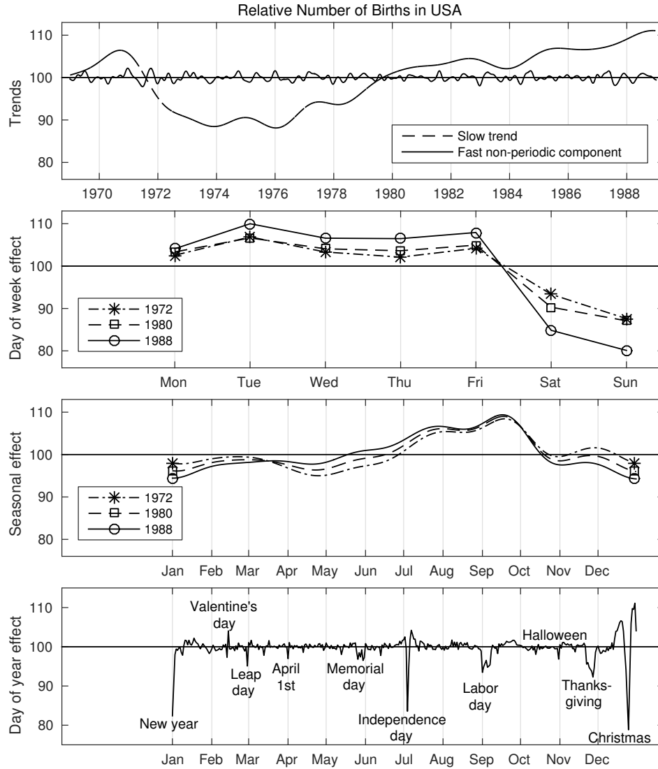
Figure 21.5 Relative number of births in the United States based on exact data from each day from 1969 through 1988, divided into different components, each with an additive Gaussian process model. Compared to Figure 21.4, this improved model allows individual effects for every day of the year, not merely for a few selected dates.
