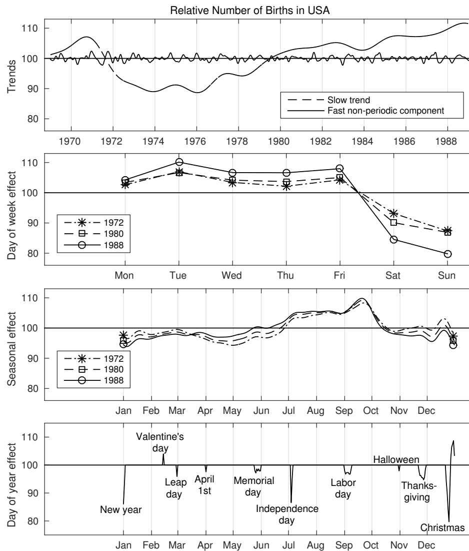
Figure 21.4 Relative number of births in the United States based on exact data from each day from 1969 through 1988, divided into different components, each with an additive Gaussian process model. The estimates from an improved model are shown in Figure 21.5.
