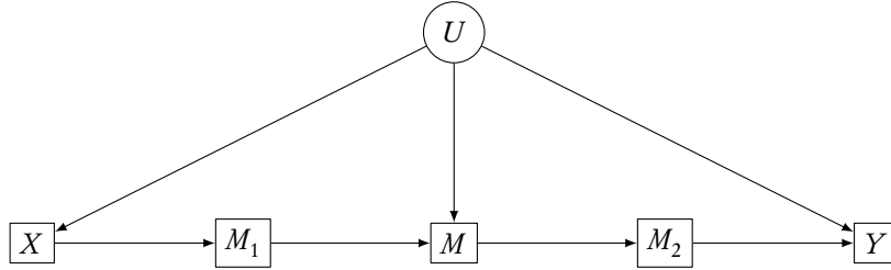
FIGURE 22.5: The path X \rightarrow M \rightarrow Y contains all the mechanisms by which X influences Y , but is not isolated from the rest of the system ( U \rightarrow M ). The sub-mechanisms X \rightarrow M_1 \rightarrow M and M \rightarrow M_2 \rightarrow Y are isolated, and the original causal effect can be identified by composing them.
