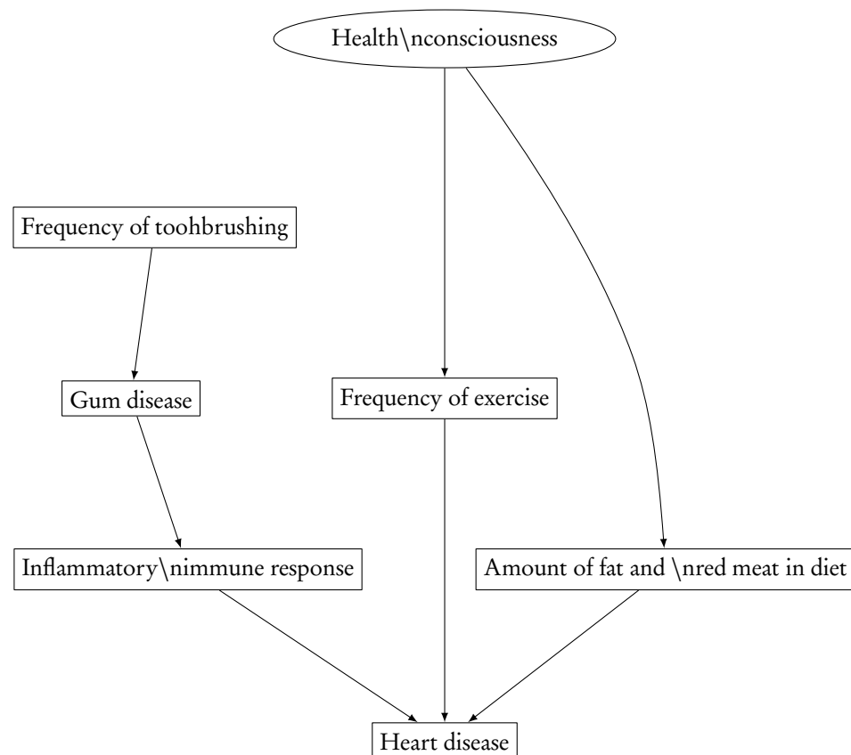
FIGURE 21.3: The previous graphical model, “surgically” altered to reflect a manipulation (do) of brushing.
