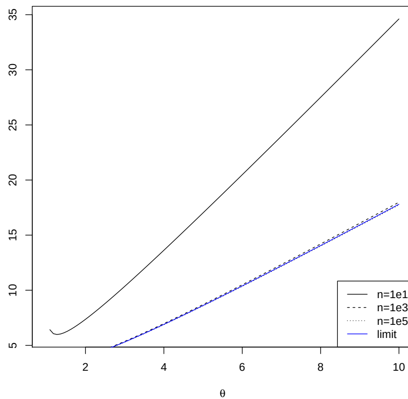
FIGURE H.5: Convergence of objective functions, here, negative average log-likelihoods. Note that the limiting, n = \infty objective function (solid blue line) is extremely close to what we see at n = 10^5 already. See Code Example 46 for code.
