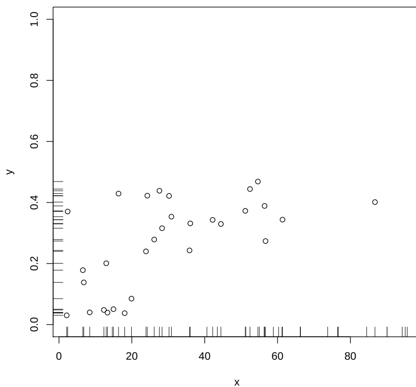
FIGURE M.1: Running example for illustrating missing-data issues. The rug-plots along the axes indicate the marginal distributions of the observed (not missing) values. The generating code is deliberately hidden here, but will be given at the end of the chapter.
