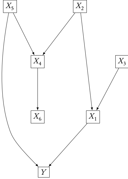
FIGURE 20.4: Example DAG used to illustrate d-separation.
