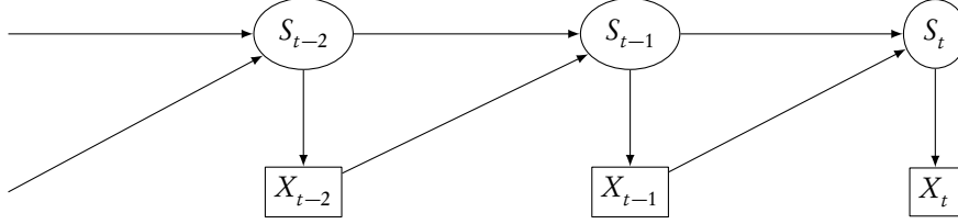
FIGURE 25.22: DAG for a chain with complete connections. The current state S_t is the only parent of the current observation X_t , and those two together are the only parents of the next state S_{t+1} . (In fact, they're usually assumed to fix S_{t+1} deterministically.) The S 's are Markovian, the X 's are not, X_t \perp\!\!\!\perp S_{-\infty:t-1}, X_{-\infty:t-1} | S_t , and X_{t+1:\infty}, S_{t+1:\infty} \not\perp\!\!\!\perp X_t | S_t .
