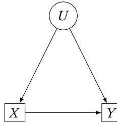
FIGURE 22.1: The distribution of Y given X , \Pr(Y|X) , confounds the actual causal effect of X on Y , \Pr(Y|do(X=x)) , with the indirect dependence between X and Y created by their unobserved common cause U . (You may imagine that U is really more than one variable, with some internal sub-graph.)
