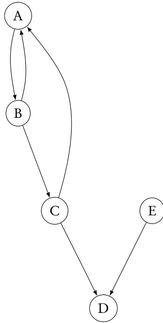
FIGURE J.1: Example for illustrating the concepts of graph theory.
