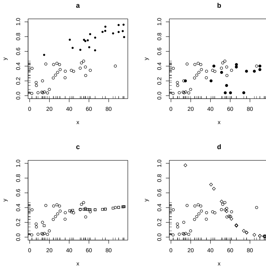
FIGURE M.2: Some possible complete data sets, all compatible with the observations in Figure M.1. The four point shapes indicate four distinct data-generating processes. In all four, the hollow circles are the fully-observed data points.
