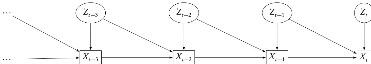
FIGURE 25.25: The DAG for an ARMA(1,1) model.
