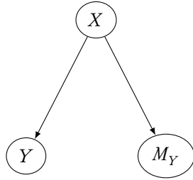
FIGURE M.4: The simplest (but not the only!) graphical model in which Y might be missing at random (MAR), but not missing completely at random (MCAR).
