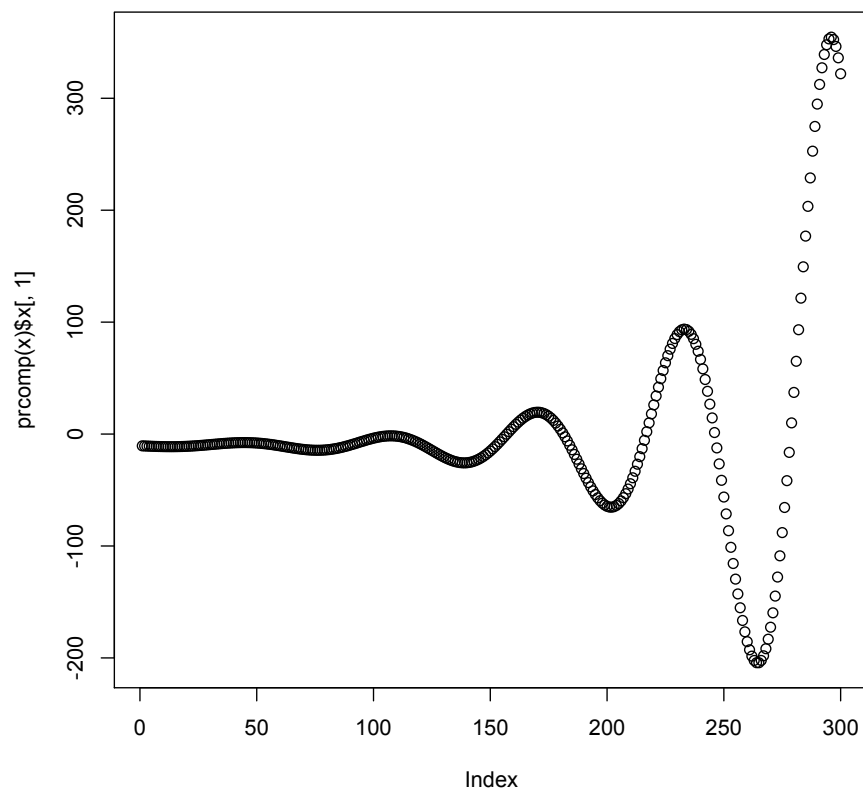
FIGURE 18.2: Projections of the spiral points on to their first principal component. [[TODO: Make code-generated figure!]]
