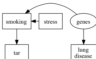
FIGURE 24.1: A hypothetical causal model in which smoking is associated with lung disease, but does not cause it. Rather, both smoking and lung disease are caused by common genetic variants. (This idea was due to R. A. Fisher.) Smoking is also caused, in this model, by stress.
