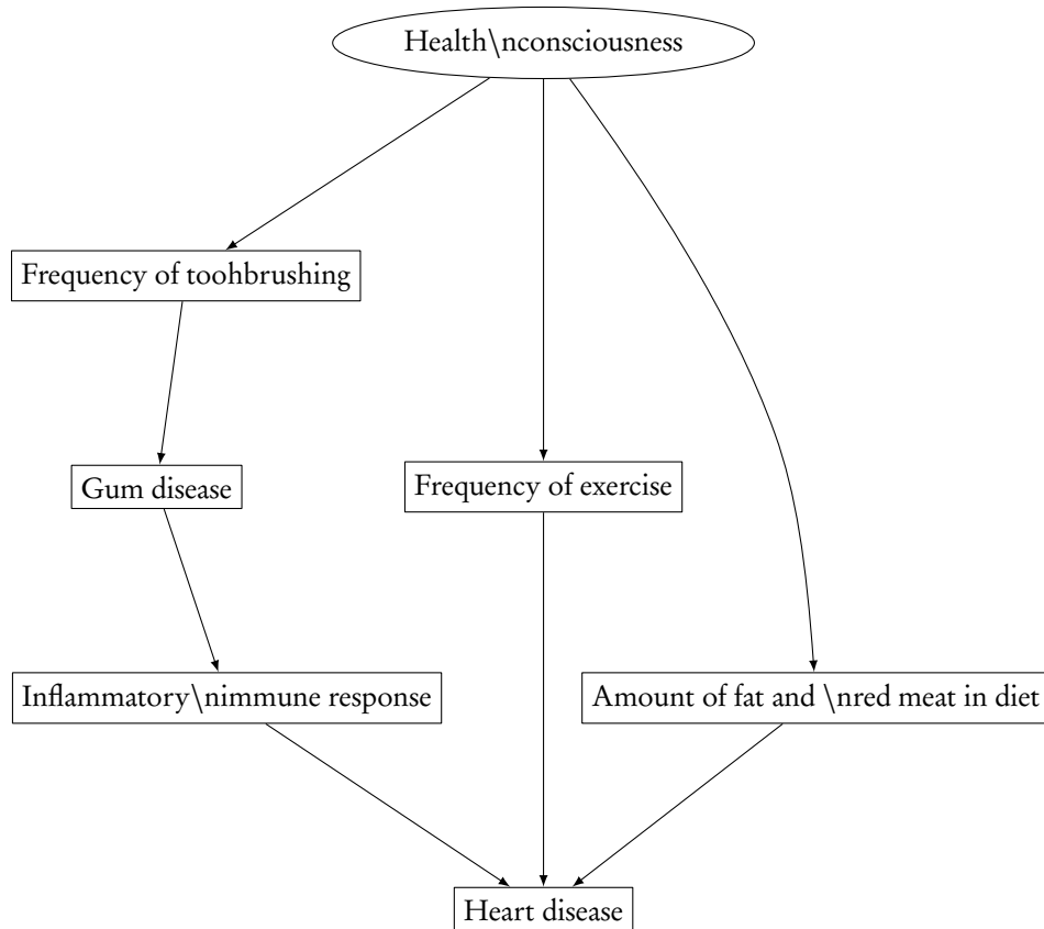
FIGURE 21.2: Graphical model illustrating hypothetical pathways linking brushing your teeth to not getting heart disease.
