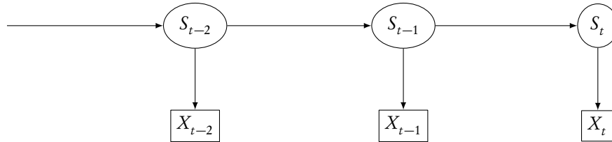
FIGURE 25.21: DAG for hidden Markov models. The current state S_t is the only parent of the current observation X_t and the only parent of the next state S_{t+1} . Thus the S 's are Markovian, the X 's are not, X_t \perp\!\!\!\perp S_{-\infty:t-1}, X_{-\infty:t-1} | S_t , and X_{t+1:\infty}, S_{t+1:\infty} \perp\!\!\!\perp X_t | S_t .
