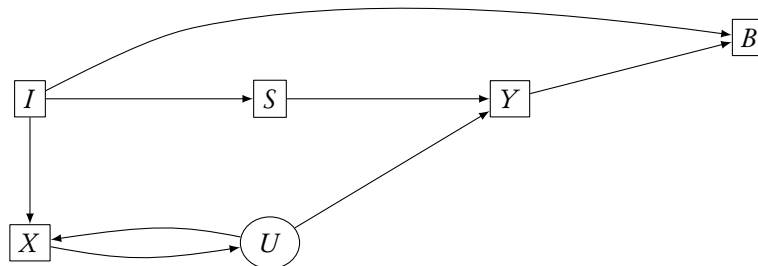
FIGURE 22.6: A valid instrumental variable, I , is related to the cause of interest, X , and influences Y only through its influence on X , at least once control variables block other paths. Here, to use I as an instrument, we should condition on S , but should not condition on B . (If we could condition on U , we would not need to use an instrument.)
