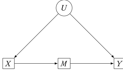
FIGURE 22.4: Illustration of the front-door criterion, after Pearl (2009b, Figure 3.5). X , Y and M are all observed, but U is an unobserved common cause of both X and Y . X \leftarrow U \rightarrow Y is a back-door path confounding the effect of X on Y with their common cause. However, all of the effect of X on Y is mediated through X 's effect on M . M 's effect on Y is, in turn, confounded by the back-door path M \leftarrow X \leftarrow U \rightarrow Y , but X blocks this path. So we can use back-door adjustment to find \Pr(Y|do(M = m)) , and directly find \Pr(M|do(X = x)) = \Pr(M|X = x) . Putting these together gives \Pr(Y|do(X = x)) .
