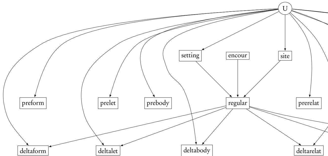
FIGURE A.1: First DAG.
