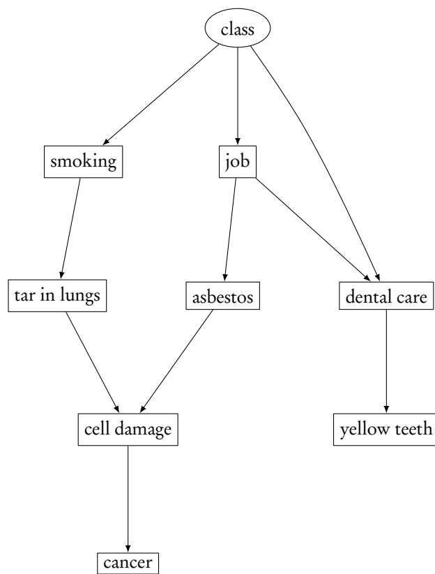
FIGURE 22.10: DAG for Exercise 3.
