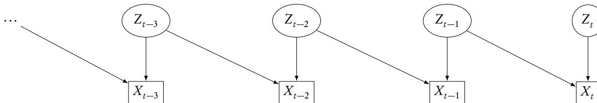
FIGURE 25.23: The DAG for a first-order moving average model.
