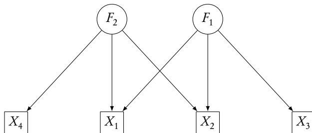
FIGURE 20.1: Illustration of a typical model with two latent factors ( F_1 and F_2 , in circles) and four observables ( X_1 through X_4 ).
