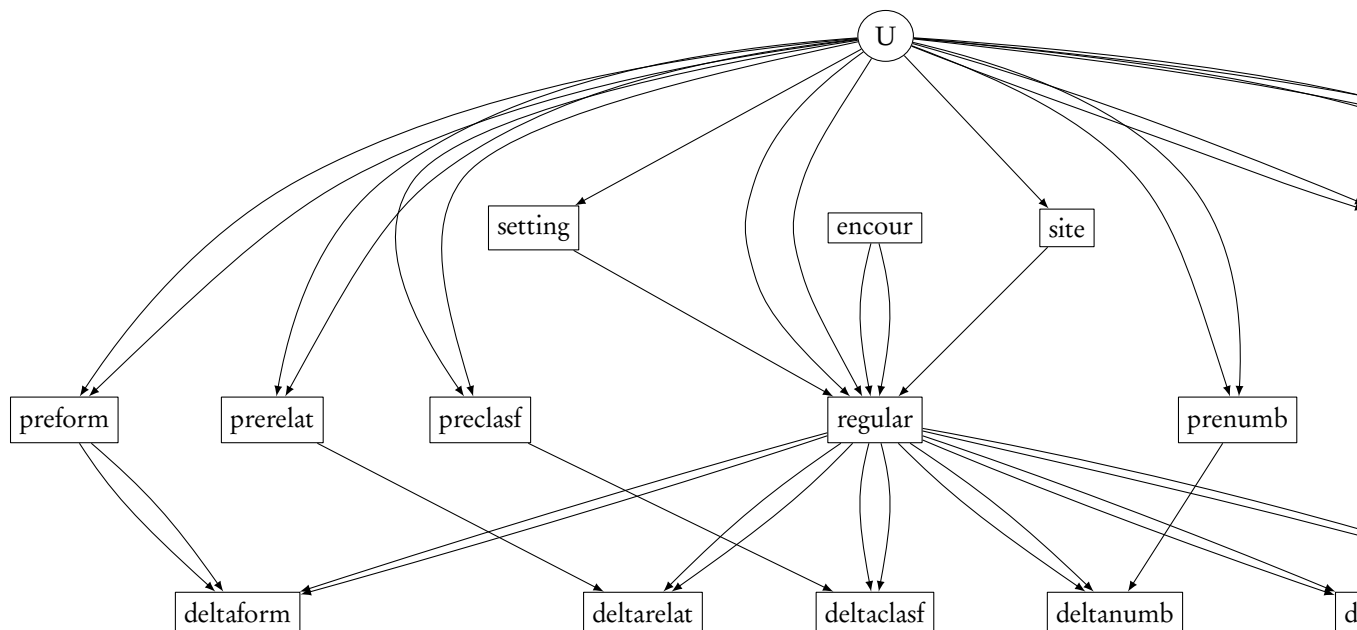
FIGURE A.2: Second DAG.
