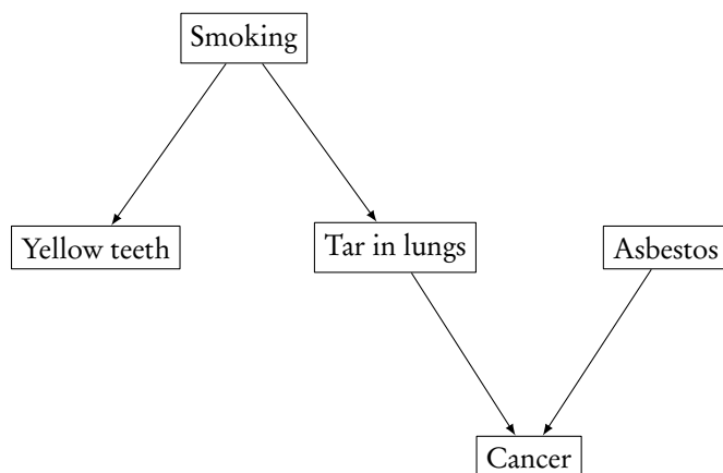
FIGURE 20.6: DAG model indicating (hypothetical) relationships between smoking, asbestos, cancer, and covariates.
