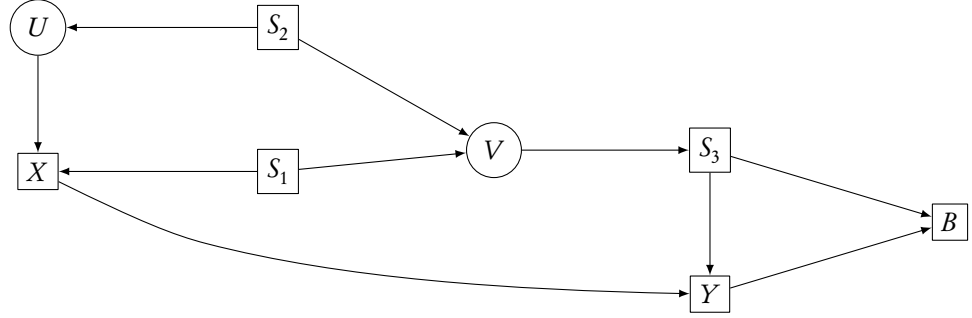
FIGURE 22.3: Illustration of the back-door criterion for identifying the causal effect of X on Y . Setting S = \{S_1, S_2\} satisfies the criterion, but neither S_1 nor S_2 on their own would. Setting S = \{S_3\} , or S = \{S_1, S_2, S_3\} also works. Adding B to any of the good sets makes them fail the criterion.
