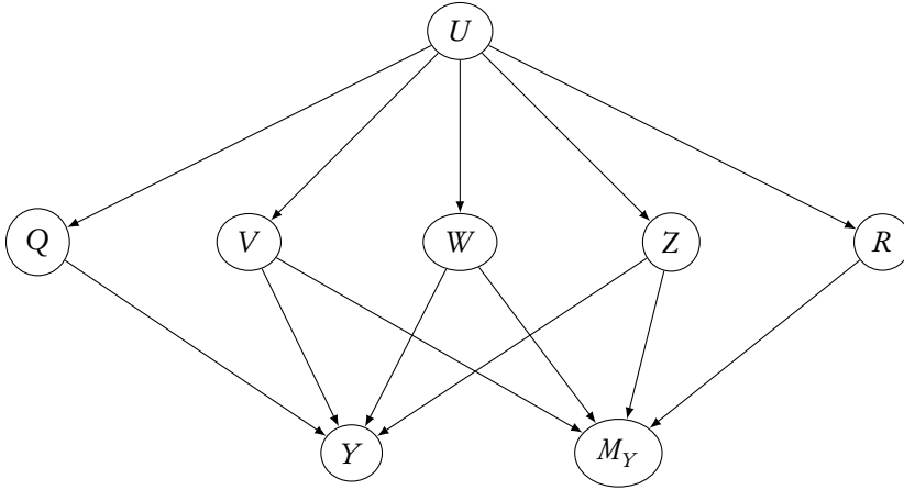
FIGURE M.5: Whether Y is missing-at-random or not can depend on the variables used for conditioning. Suppose that whether or not a student is admitted (or a loan approved, or an arrestee released) depends on X = \{V, W, Z, R\} , and Y is some measure of academic success (or loan repayment, or subsequent trouble with the law). Then Y \perp\!\!\!\perp M_Y | X , and Y is missing-at-random for the decision-makers. But we as data-analysts might only have access to X' = \{V, W, Q\} , and then Y \not\perp\!\!\!\perp M_Y | X' . See Exercise 4 for proofs and extensions.
