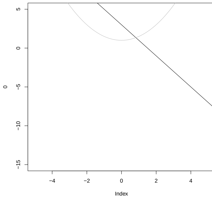
FIGURE 10.1: Black line: Linear response function ( y = 3 - 2x ). Grey curve: standard deviation as a function of x ( \sigma(x) = 1 + x^2/2 ). (Code deliberately omitted; can you reproduce this figure?)
