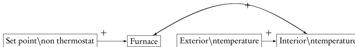
FIGURE 20.7: Directed but cyclic graphical model of a feedback loop. Signs (+, – on arrows are “guides to the mind”. Cf. Figure 20.8.
